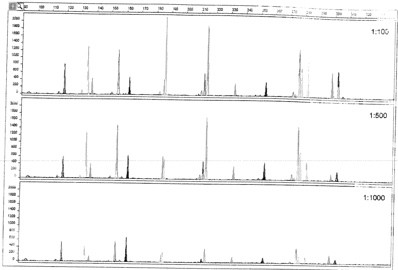
FIG. 8—Mixture studies of male and female blood samples. Profiles shown in the panels from top to bottom correspond to the samples extracted from the cotton swab containing 1 \mu L of male blood combined with 100, 500, and 1000 \mu L of female blood, respectively.
