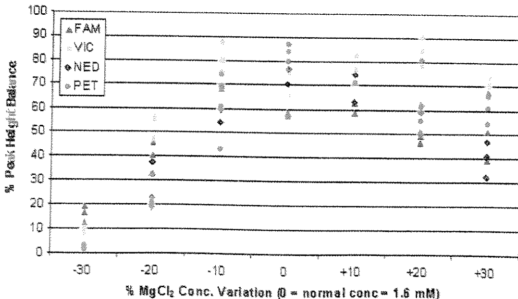
FIG. 2—Effect of MgCl 2 titration on the intracolor peak balance of 1 ng male control DNA 007. Samples were amplified with PCR reaction mixes at ± 10%, 20%, and 30% of the optimal 0% (1.60 mM) and resolved on an ABI PRISM® 3100 genetic analyzer. The MgCl 2 concentrations tested were: 1.12 mM (-30), 1.28 mM (-20), 1.44 mM (-10), 1.60 mM (0), 1.76 mM (+10), 1.92 mM (+20), and 2.08 mM (+30). The peak height balance from loci in the same color were averaged and shown as data points (n = 3).
