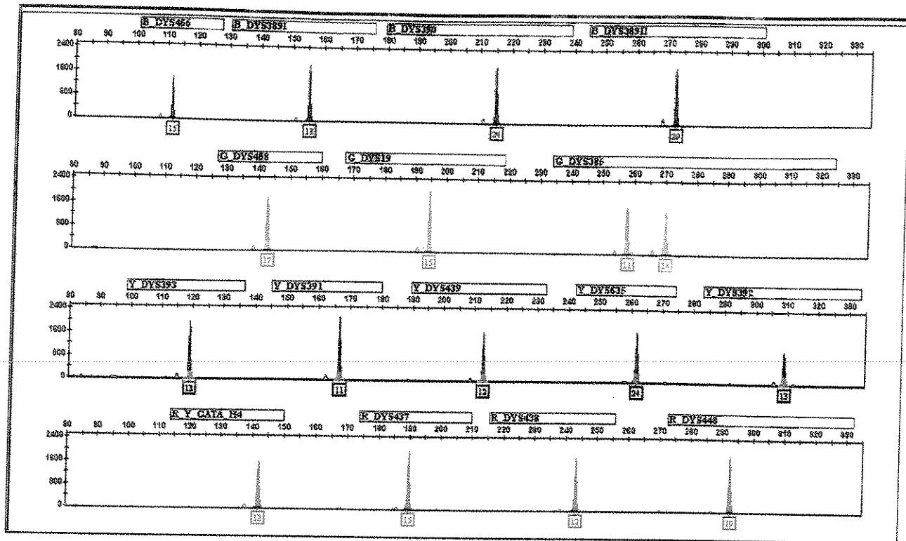
FIG. 1—Representative electropherogram from GeneMapper® ID software v3.2 showing the profile of 1 ng of AmpFℓSTR® control DNA 007 amplified with the Yfiler™ kit. The four panels correspond to 6-FAM™, VIC®, NED™, and PET® dye-labeled peaks. The haplotype is shown with the allele number displayed underneath each peak.
