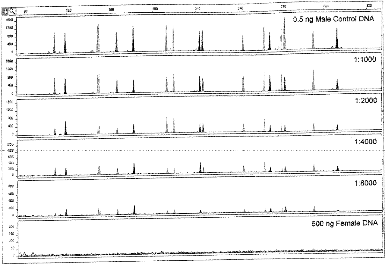
FIG. 7.—Mixture studies. Amplification of male control DNA 007 in the presence of female DNA 9947A. Profiles shown in the panels from top to bottom: 500 pg of male DNA, 500 pg male DNA with 500 ng female DNA (1:1000), 250 pg male DNA with 500 ng female DNA (1:2000), 125 pg male DNA with 500 ng female DNA (1:4000), 63 pg male DNA with 500 ng female DNA (1:8000), and 500 ng female DNA.
