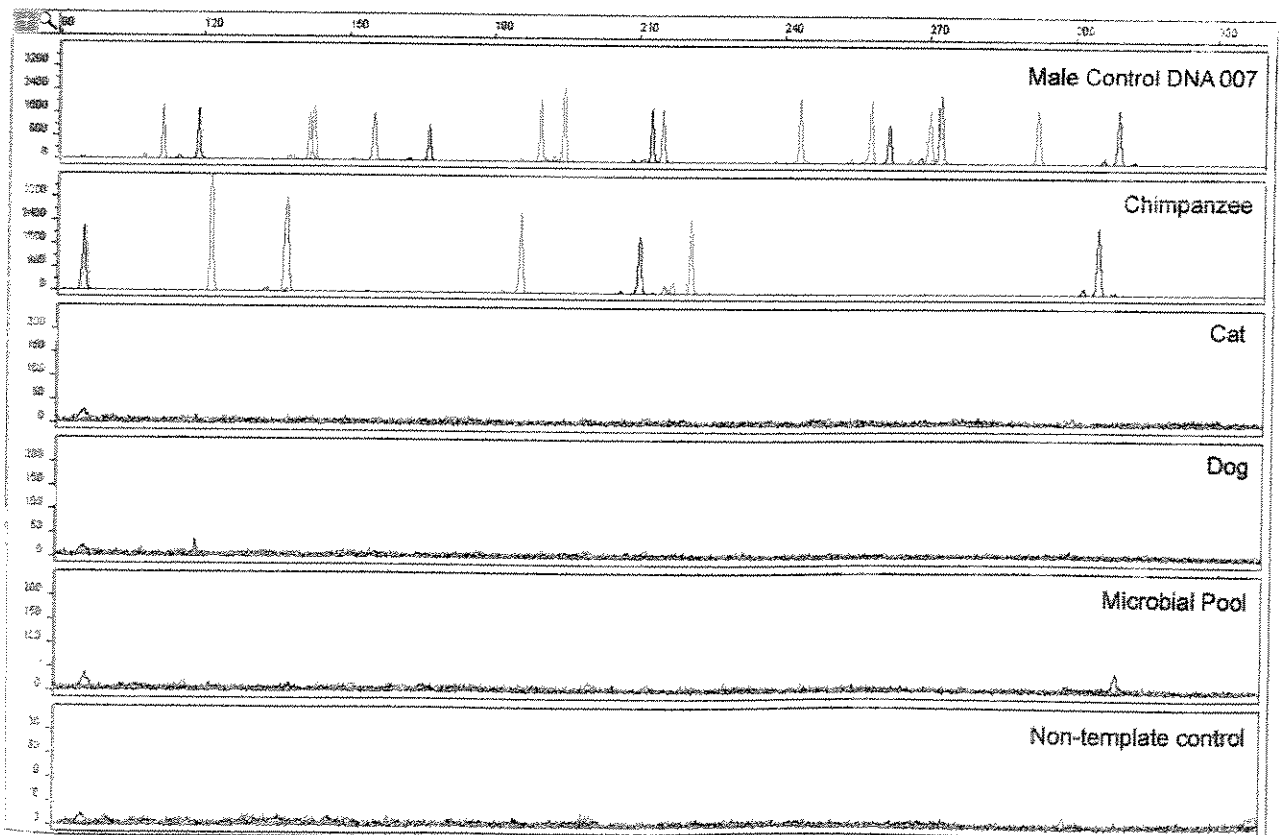
FIG. 4—Representative electropherograms from a species specificity study. From top to bottom: 1 ng of the AmpFLSTR® control DNA 007 (human), 1 ng of chimpanzee DNA, 10 ng of cat DNA, 10 ng of dog DNA, microbial pool (approx. 100,000 copies each of Candida albicans , Escherichia coli and Lactobacillus amplified together) and a nontemplate control (NTC).
